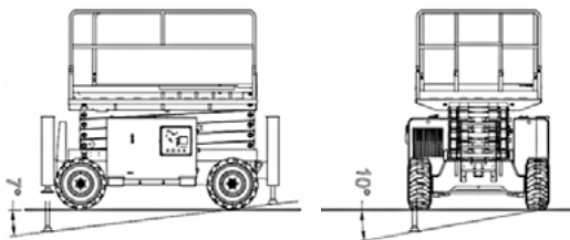
Max. outrigger leveling (front to back / side to side)
